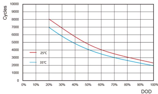
DOD vs. Cycles
