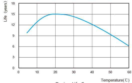
Design Life Curve
